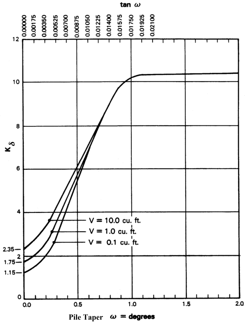
Figure 9-10. Design curves for evaluating K_\delta for piles when \phi = 35^\circ (after Nordlund, 1963).
