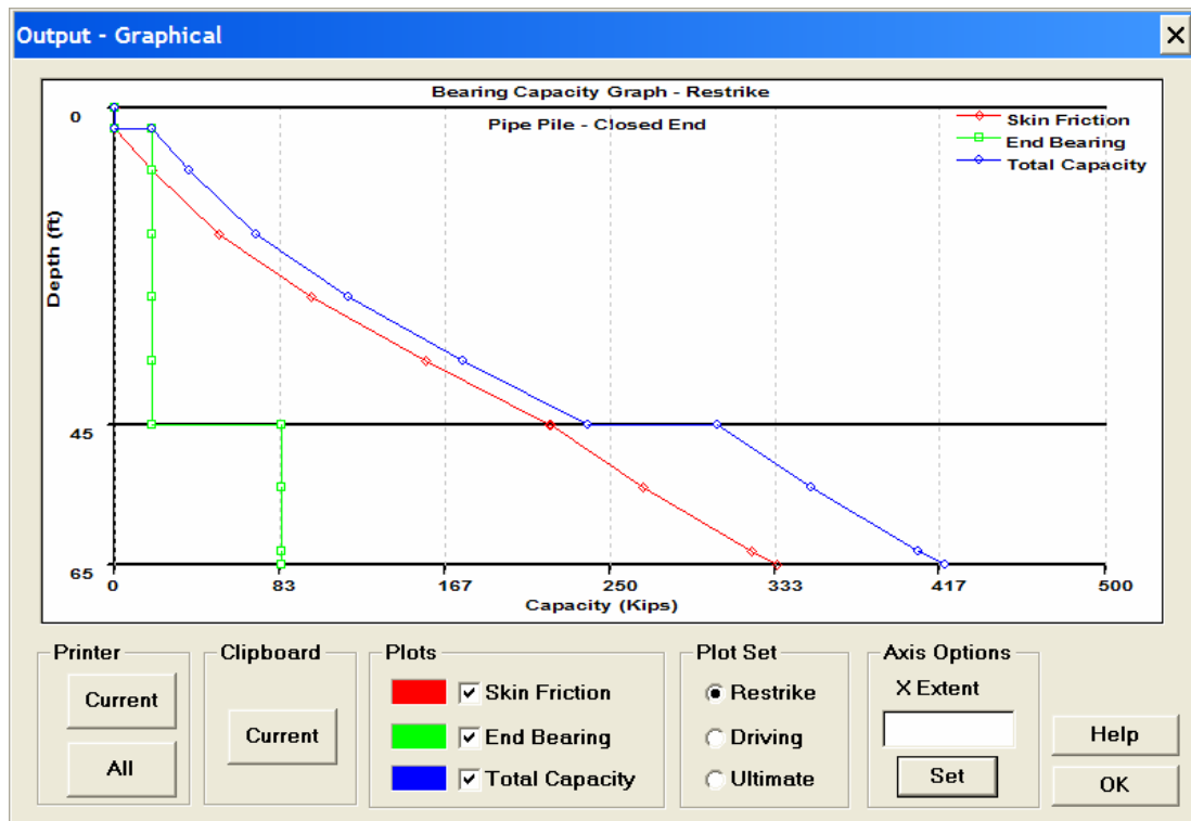
Figure 9-30. DRIVEN Output -Graphical screen for restrike.
