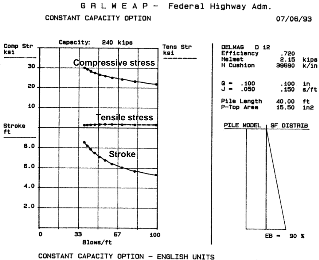
Figure 9-43. Graph of diesel hammer stroke versus blow count for a constant pile capacity.
