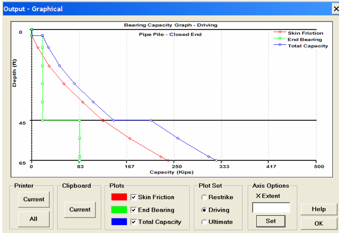
Figure 9-29. DRIVEN Output-Graphical screen for end of driving.
